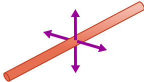
Cylindrical Symmetry
