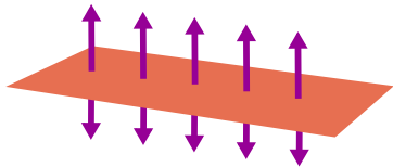
Planar Symmetry
