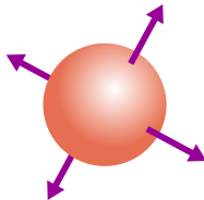
Spherical Symmetry
